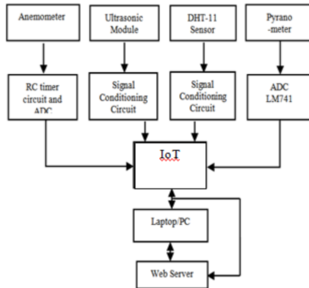
Figure.2. Block diagram of IoT based DAS
