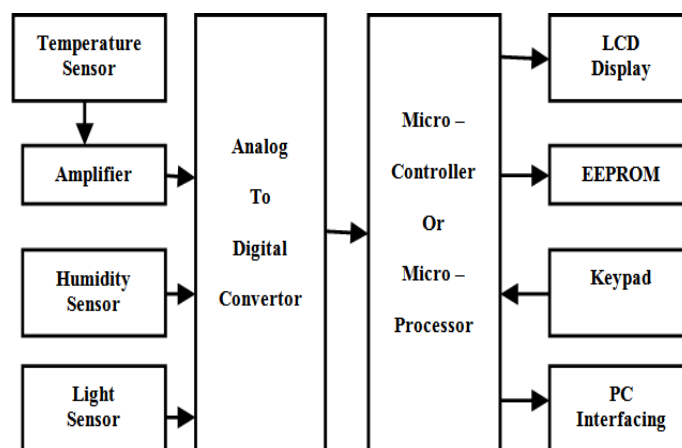
Figure.1. Basic data accession system
